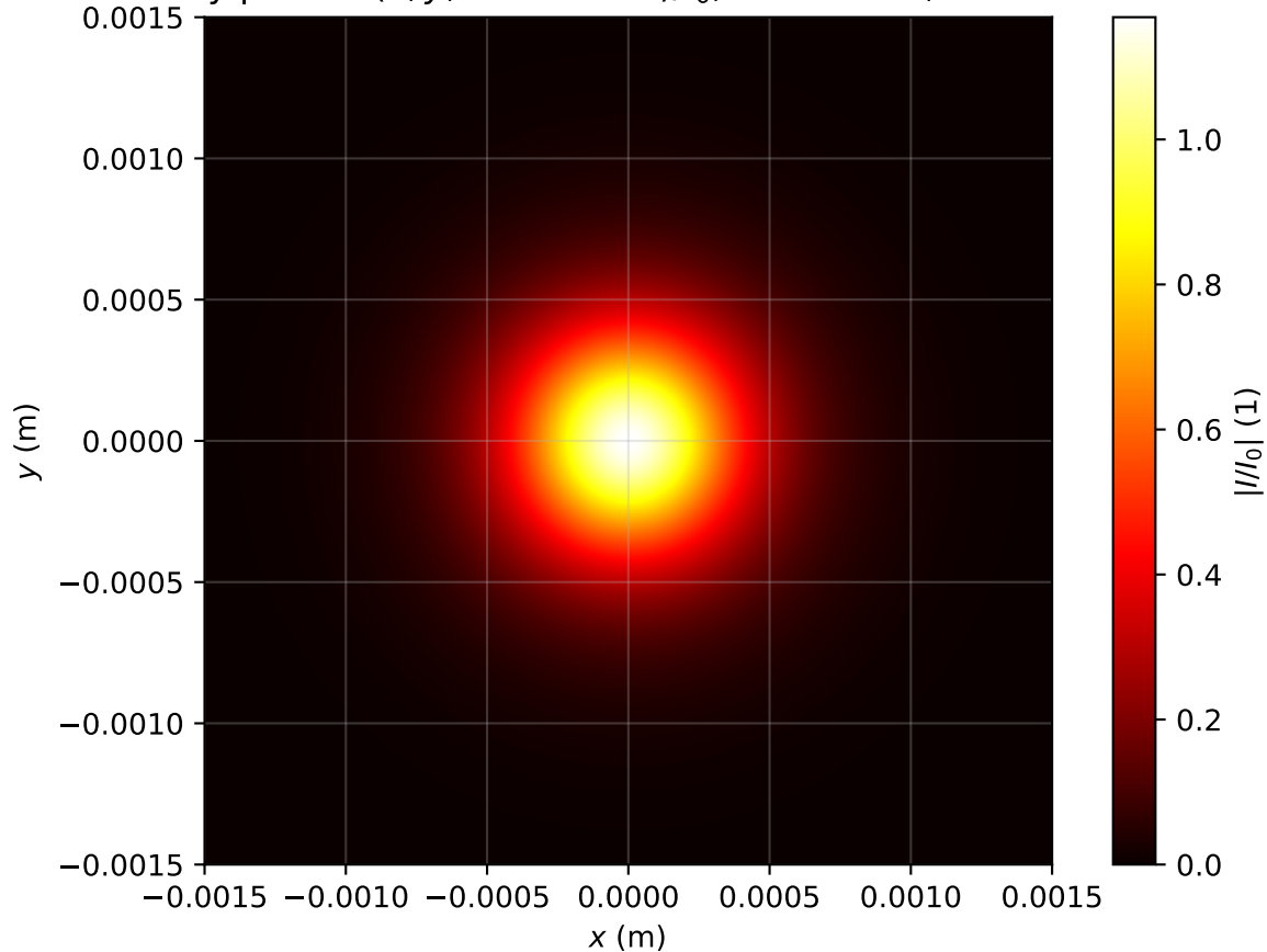
Intensity profile I(x, y, z = 1.672m)/I_0 , P_{in}=0.7P_{cr} , artificial time
